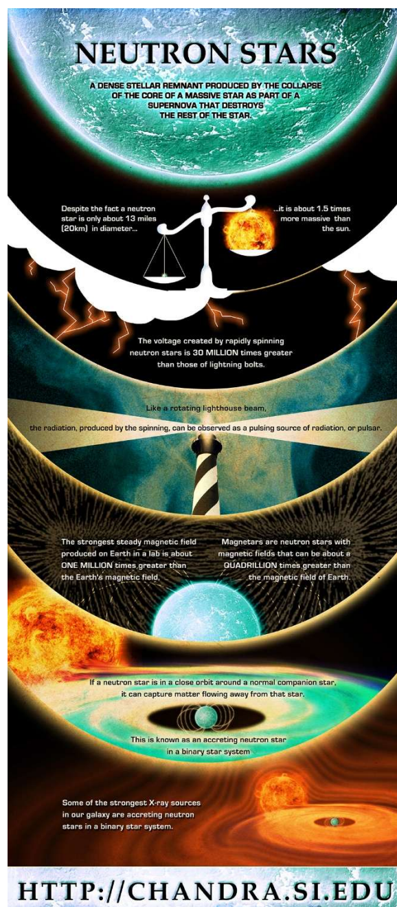
Figure 7; Interesting facts about neutron stars
