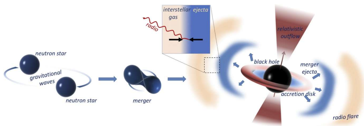
Figure 6; Neutron stars merging
